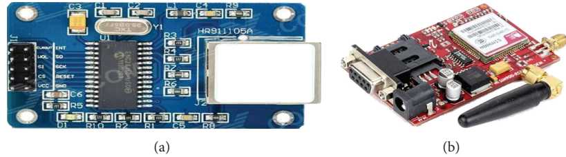
FIGURE 10: (a) ENC28J60 Ethernet module and (b) Sim900 GSM/GPRS module.
