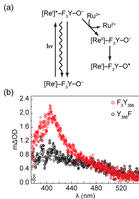
Figure 2. (a) Scheme describing the photochemistry of F_3Y generation; (b) TA spectra collected 3 \mu s after 355 nm excitation of 50 \mu M [Re]^{III}\text{-}F_3Y_{356}\text{-}\beta_2 (red) or [Re]^{III}\text{-}Y_{356}F\text{-}\beta_2 (black), and 75 \mu M \alpha_2 , 1 mM CDP, 3 mM ATP, and 10 mM Ru(NH_3)_6Cl_3 , in assay buffer at pH 8.2.
