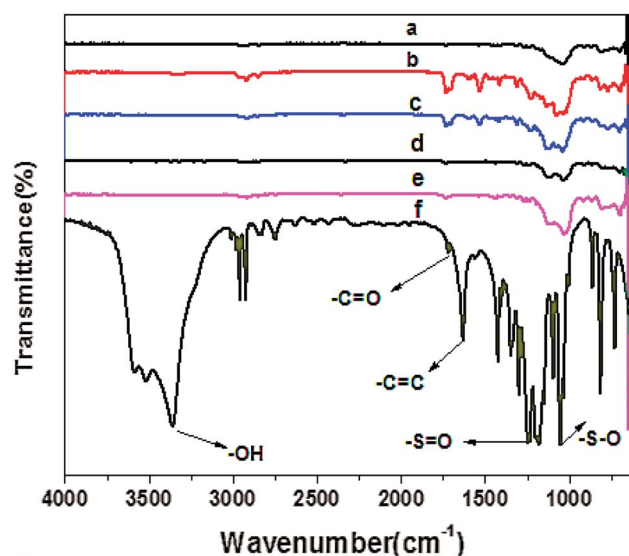
Fig. 3 (a) FTIR of PU-Si, (b) FTIR of PU-Si- g -P(DMCHPS)-12 h, (c) FTIR of PU-Si- g -P(DMCHPS)-24 h, (d) FTIR of PU-Si- g -P(DMCHPS)-36 h, (e) FTIR of PU-Si- g -P(DMCHPS)-48 h, (f) FTIR of DMCHPS.
