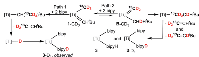
Scheme 3 Isotopic labelling studies using 1 - ^{13}\text{C} and 1 - \text{D}_3 (labelled 1 - ^{13}\text{C}_3 for simplicity) with two equiv. of bipy. The role of bipy and PNP are not shown for clarity ([Ti] = (PNP)Ti).
