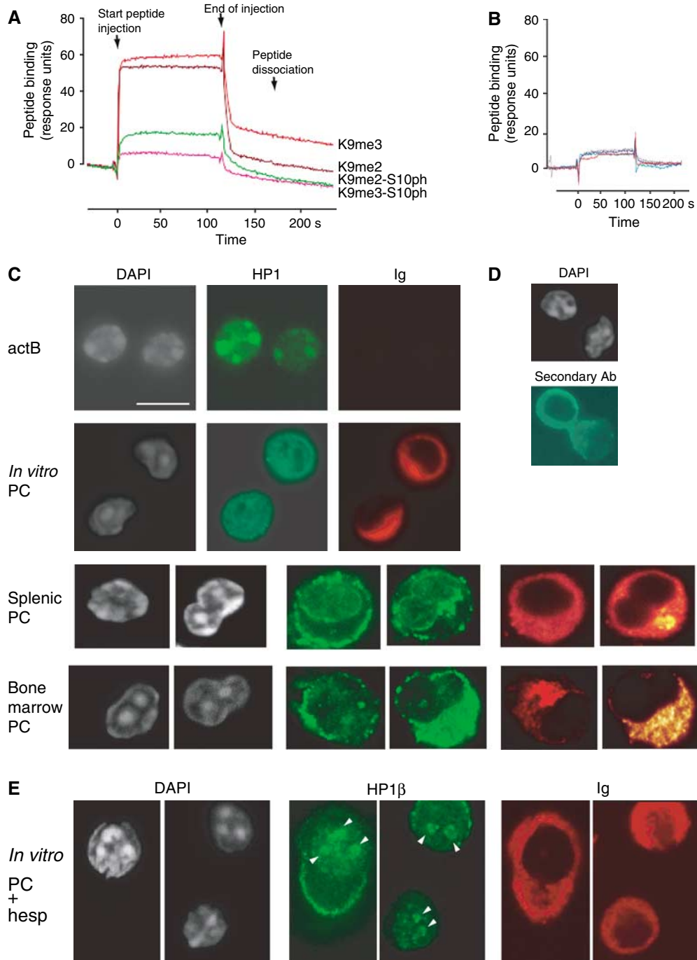
Figure 5 HP1 \beta is relocated away from heterochromatin in plasma cells. (A) Surface plasmon resonance (SPR) analysis of binding of His-HP1 \beta to peptides corresponding to aa 1–15 of histone H3 with the indicated modifications. Peptides (50 \mu M) were injected over His-HP1 \beta immobilised on a Biacore flow cell. The presence of phosphorylated S10 reduces the affinity of HP1 \beta for peptides containing both K9me3 and K9me2. (B) Nonspecific binding of the peptides to the chip when injected over a flow cell control lacking HP1 \beta . (C) Distribution of HP1 \beta relative to DAPI-intense regions in activated B and plasma cells. The analysis was carried out on plasma cells that were either differentiated in vitro ( in vitro PC), isolated from the spleen of LPS-immunised mice (splenic PC) or isolated from the bone marrow of ovalbumin-immunised mice (bone marrow PC). (D) Staining of plasma cells with the Alexa 488 \alpha -rat secondary antibody alone showed some crossreactivity with the mouse immunoglobulin (Ig) in the cytoplasm but not the nucleus. (E) Incubation of plasma cells in a medium containing 200 nM hesperadin for 1.5 h results in relocalisation of HP1 \beta to heterochromatin (indicated by arrows) in 29% of the cells.
