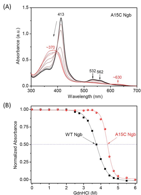
Fig. 4 UV-Vis spectra of Gdn·HCl-induced unfolding of (A) A15C Ngb (10 \mu M protein in 100 mM potassium phosphate buffer, pH 7.0). (B) Normalized absorbance of the Soret band versus Gdn·HCl concentrations.
