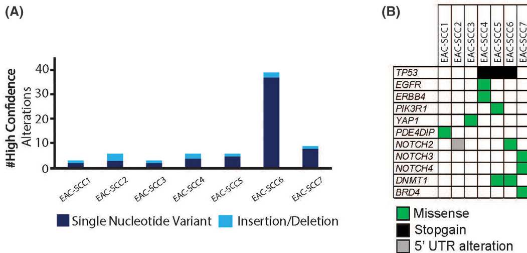
FIGURE 1 Frequency distribution of high-confidence somatic mutation and copy number alteration calls (A), and frequently mutated genes (B) in our seven external auditory canal (EAC) squamous cell carcinomas (SCC) tumors
