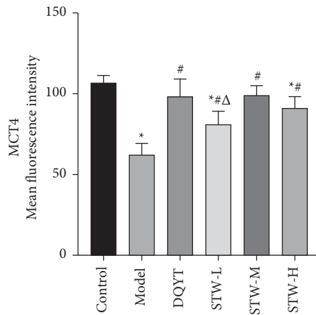
FIGURE 8: Effects of STW on the expression levels of GLUT1 and MCT4 proteins in mouse trophoblasts (40×): (a) GLUT1 immunohistochemistry staining in trophoblasts; (b) MCT4 immunohistochemistry staining in trophoblasts; (c–d) GLUT1 and MCT4 protein levels in trophoblasts. Compared with the control group, * P < 0.05 ; compared with the model group, # P < 0.05 ; compared with the DQYT group, \Delta P < 0.05 .
