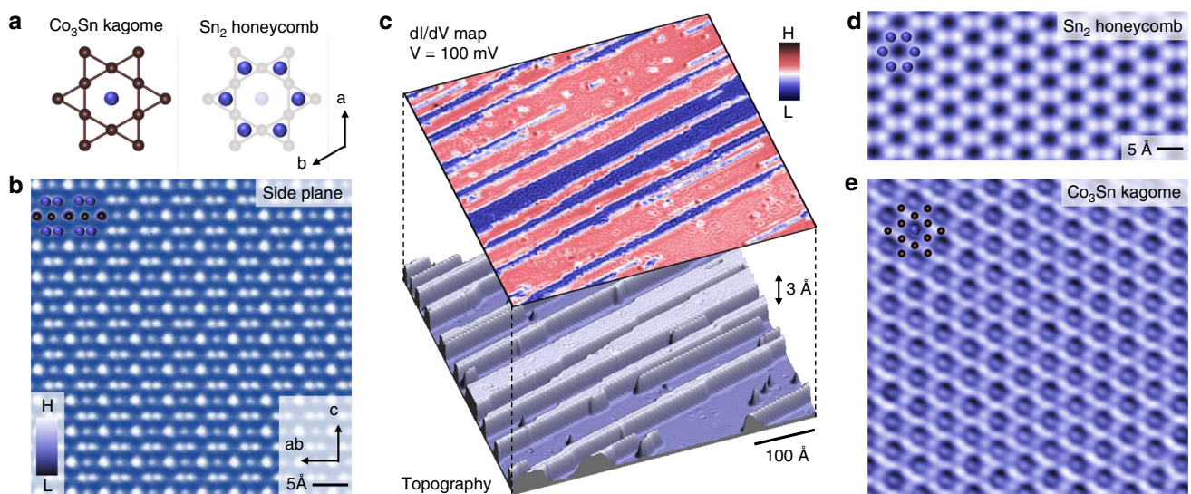
Fig. 1 Complete atomic-scale visualization of kagome lattice in CoSn. a Crystal structure of CoSn, which consists of a Co 3 Sn kagome layer (left) and a Sn 2 honeycomb layer (right). b Cross-sectional atomic resolution scanning transmission electron microscope image of CoSn, showing the lattice stacking along the c axis as illustrated in the inset. c Topographic image of a single atomic step (bottom) and the corresponding differential conductance map obtained at a bias voltage of 100 mV (top). d Atomically resolved Sn 2 surface with the corresponding atomic lattice structures. e Atomically resolved Co 3 Sn surface with the corresponding atomic lattice structures.
