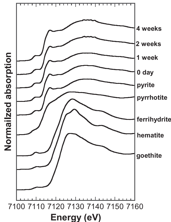
Fig. 6. Iron K-edge XANES spectra of bulk solid samples after incubations and Fe model compounds of pyrite, pyrrhotite, ferrihydrite, hematite, and goethite.
