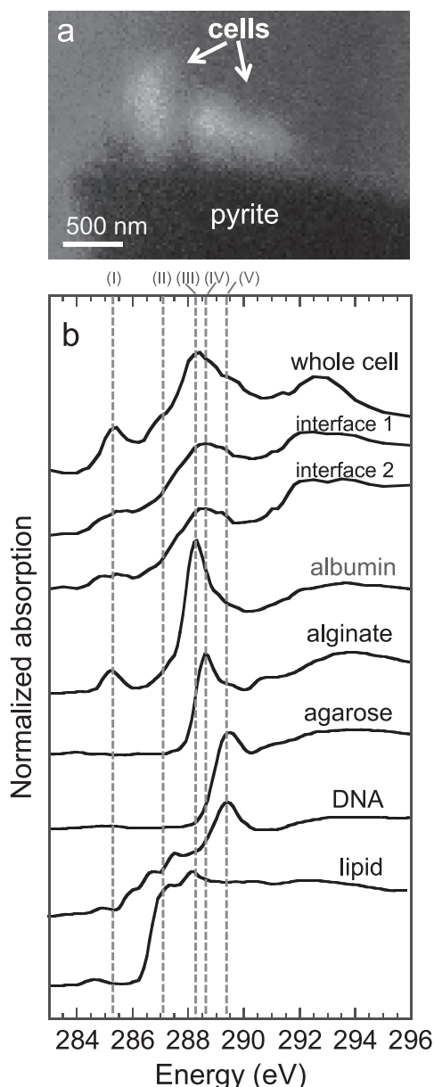
Fig. 3. (a) STXM-based C image of sessile A. ferrooxidans cells on pyrite in the 2-week incubation. The image was obtained by dividing the two images at 282 eV (C 1s pre-edge energy) and 304 eV (post-edge energy). (b) STXM-based C 1s NEXAFS spectra of model compounds and sessile A. ferrooxidans cells. In C NEXAFS, sodium alginate (acidic polysaccharide), agarose (neutral polysaccharide), albumin (protein), Escherichia coli DNA (nucleic acid), and 1,2-dipalmitoyl-sn-glycero-3-phosphoethanolamine (lipid) were selected as model compounds for major microbial biomolecules, as in previous studies (5, 8). The dotted lines (I) to (V) in Fig. 3b stand for the peak energies of the major organic functional groups present in the model compounds shown in Table 1.
