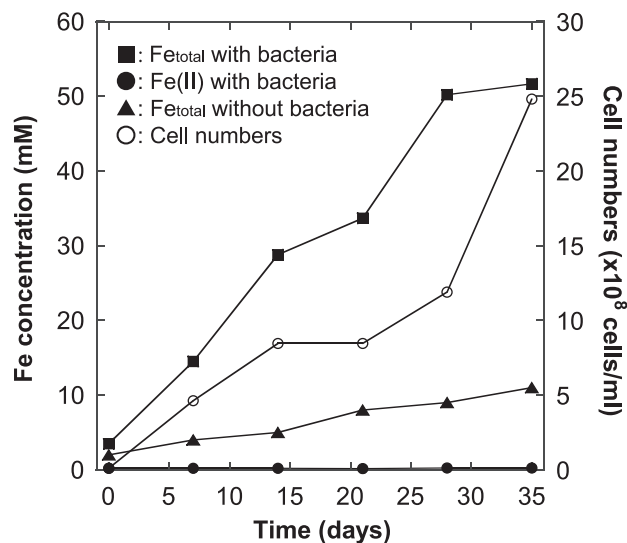
Fig. 1. Concentrations of total Fe and Fe(II) with/without bacteria and cell numbers. The initial amount of pyrite was 0.5 g in a total volume of 10 mL at an initial pH 3.
