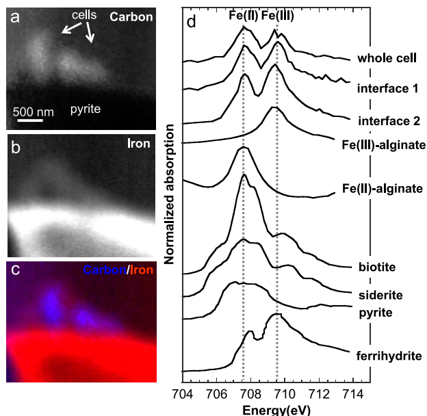
Fig. 5. STXM-based C, Fe, and merged images (a, b, c) and Fe 2p NEXAFS spectra (d) of model compounds and sessile A. ferrooxidans cells on pyrite after a 2-week incubation. Pyrite, ferrihydrite, siderite, biotite, and Fe(II) and Fe(III) complexed with acidic polysaccharides (sodium alginate) were selected as the model compounds for Fe NEXAFS. Vertical lines in Fig. 5d were displayed to show the specific Fe(II) and Fe(III) peaks at 707.5 and 709.1 eV, respectively. The Fe image was obtained by dividing two images at 700 eV (Fe 2p pre-edge energy) and 730 eV (post-edge energy).
