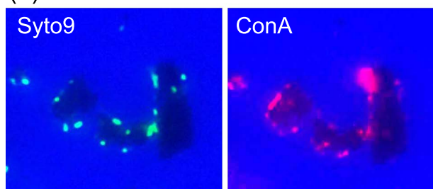
Fig. 4. Sessile A. ferrooxidans cells on pyrite particles stained with Syto9 for nucleic acids, and with ConA for extracellular polysaccharides after incubations for 2 weeks (a) and 4 weeks (b). Black grains in the images show pyrite particles. All scale bars: 10 \mu m.
