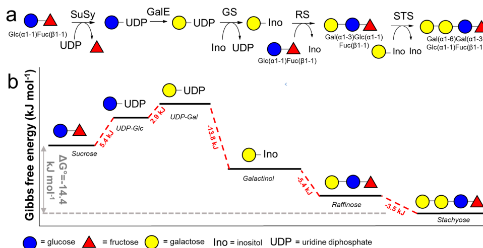
Figure 7. Enzymatic cascade for the production of stachyose from sucrose with glycosyltransferases. (a). The standard Gibbs free energy changes of the individual reactions ( \Delta_rG^\circ s, red) and the total reaction ( \Delta_rG^\circ , grey) shown in (b) [183]. The \Delta_rG^\circ represents the change of Gibbs free energy and was calculated using the eQuilibrator web interface ( http://equilibrator.weizmann.ac.il ) [155] using the following conditions: ionic strength 0.1 M, pH 7.0, 1 mM of component, 298 K. Abbreviations: UDP-D-glc, UDP-D-glucose; UDP-D-gal, UDP-D-galactose, SuSy, Sucrose synthase; GalE, UDP-D-glucose-4-epimerase; GS, galactinol synthase; RS, raffinose synthase; STS, stachyose synthase.
