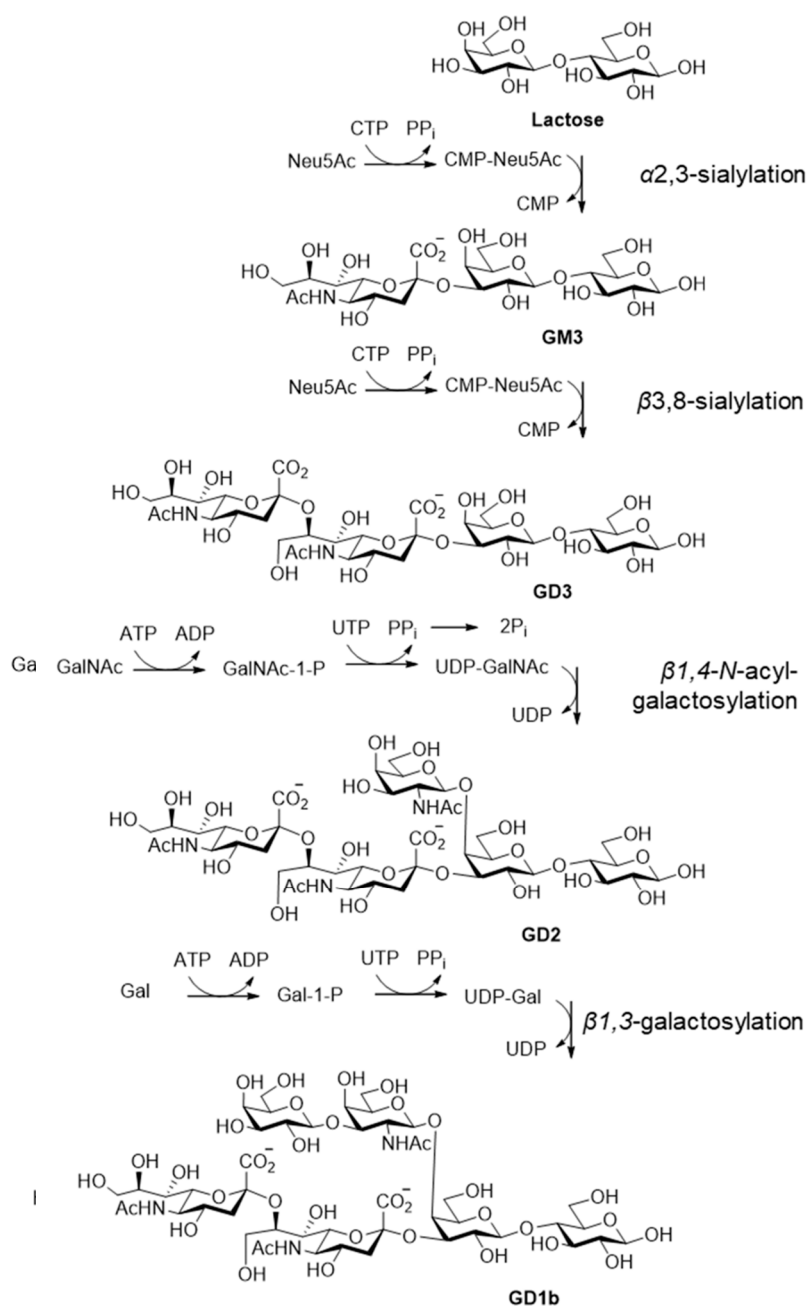
Figure 12. The enzymatic synthesis of GD1b glycan using OPME \alpha 2,3 -sialylation, \alpha 3,8 -sialylation, \beta 1,4 -N-acylgalactosylation, and \beta 1,3 -galactosylation with a sacrificial (re)generation system for N-acetylneuraminic acid (Neu5Ac), N-acetylgalactosamine (GalNAc), and D-galactose (Gal).
