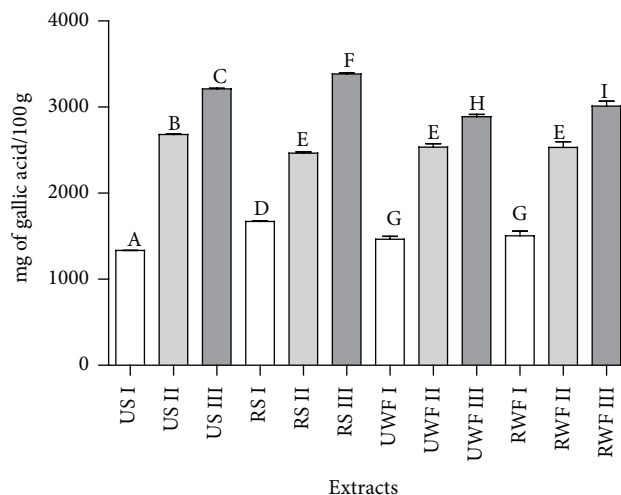
FIGURE 1: Total phenolic compounds of cocoa nibs unroasted slates (US), roasted slates (RS), unroasted well fermented (UWF) cocoa, and roasted well fermented (RWF) cocoa. Extracting solutions: I, methanol; II, methanol 50%; III, 1/2 50% methanol:1/2 70% acetone. Means with different letters differ significantly ( p < 0.05 , Tukey's test).
