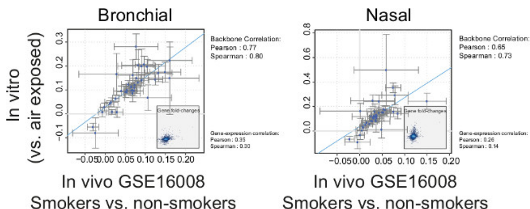
Figure 5. Network-based systems biology approach for the impact assessment of CS exposure in the context of xenobiotic metabolism. The changes of gene expressions levels were used to compute the activation of backbone node of the Xenobiotic Metabolism network model (A) as reported in a previous publication 15 . The figure on the right illustrates the concept of the quantification of the backbone nodes, also known as “differential network backbone value,” using the NPA approach. The blue ovals represent the activity of the backbone nodes ( i.e. , the functional layer) and the green balls represent the expression of genes ( i.e. , the transcriptional layer). Impacts of CS exposure in organotypic bronchial tissues ( in vitro , CS-exposed vs. air-exposed) at the 48 h of postexposure were compared to those of smoking on human bronchial epithelial collected by bronchoscopy and nasal epithelial by brushing the inferior turbinate (GSE16008) ( in vivo , smokers vs. nonsmokers) (B). Insets, correlation of the gene expression changes between the in vitro and in vivo datasets. Abbreviations: CS, cigarette smoke; NPA, network perturbation amplitude. Please click here to view a larger version of this figure.
