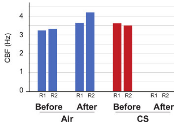
Figure 3. Cilia Beating Frequency. Cilia beating frequency (CBF) was measured in air-exposed and in the culture before and after exposure. Decreased CBF was seen after CS exposure (representative results from two insert are shown as replicate 1 (R1) and replicate 2 (R2)).
