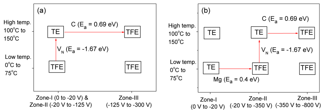
Figure 13. Change of CM with voltage zones and temperature ranges in SBDs with (a) 15 \mu\text{m} DL and (b) 30 \mu\text{m} DL. Adapted from [58] A. Sandupatla et al. 2020 Appl. Phys. Exp. https://doi.org/10.35848/1882-0786/ab93a0 . Copyright [2020] by Japanese Society of Applied Physics.
