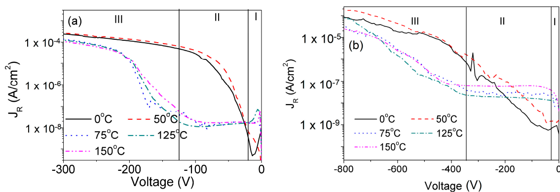
Figure 12. I–V–T characteristics of vertical GaN SBDs with (a) 15 \mu\text{m} DL, (b) 30 \mu\text{m} DL. Adapted from [58] A. Sandupatla et al. 2020 Appl. Phys. Express in press https://doi.org/10.35848/1882-0786/ab93a0 . Copyright [2020] by Japanese Society of Applied Physics.
