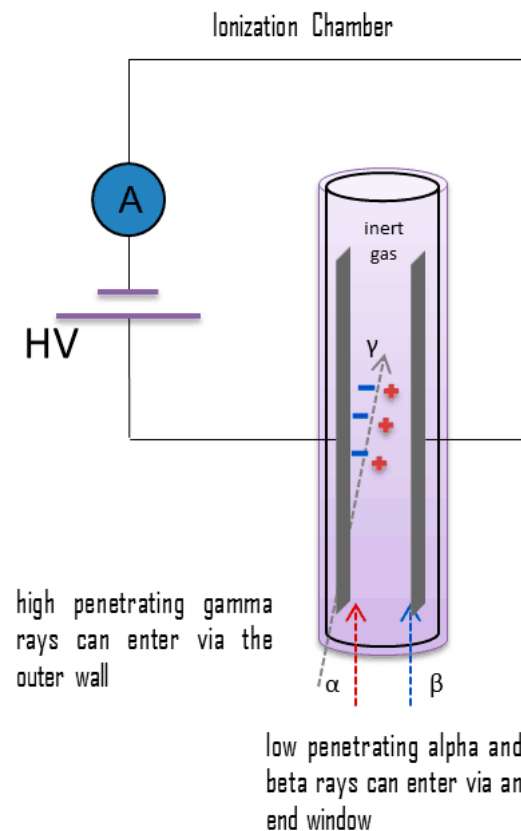
Figure 1. Schematic set-up of an Ionization detector [2,3].
