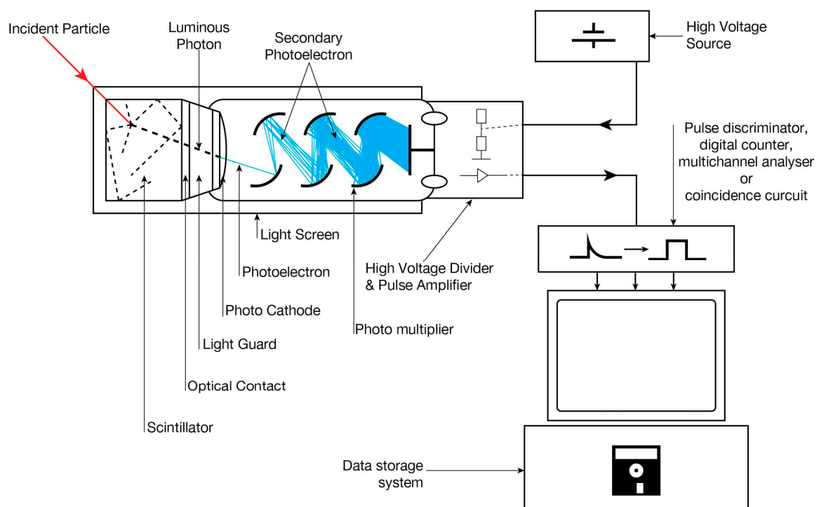
Figure 2. Schematic set-up of a Scintillation detector [3].
