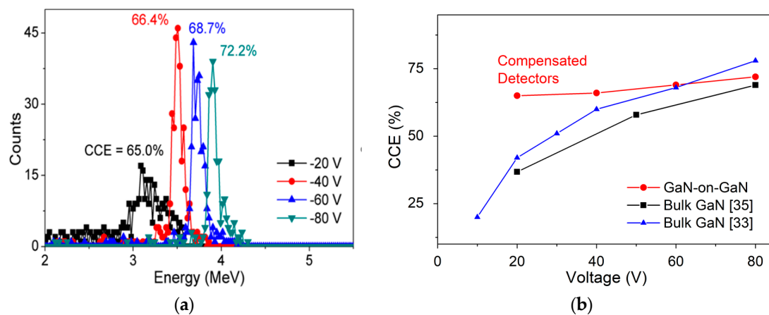
Figure 17. (a) Acquired \alpha -particle spectra of compensated detectors for different voltages ( -20 V to -80 V) and (b) Comparison of variation in CCE with voltages ( -20 V to -80 V) for state-of-the-art \alpha -particle detectors.
