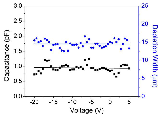
Figure 11. Variation of capacitance and DW with voltage of 0.5 mm diameter GaN SBDs with 15 \mu\text{m} .
