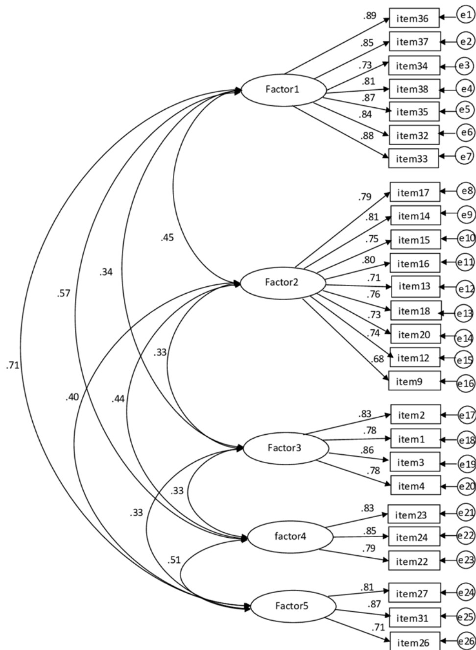
Figure 1 Confirmatory factor analysis for the Home Nursing Scale to Help Spousal Caregivers, showing the Spearman's rank correlation coefficients between each item and factor. Item numbers refer to those of the initial, 38-item scale, e-numbers refer to the new order of the items in the final, 26-item scale. CFI, comparative fit index; RMSEA, root mean square error of approximation; TLI, Tucker-Lewis index.
