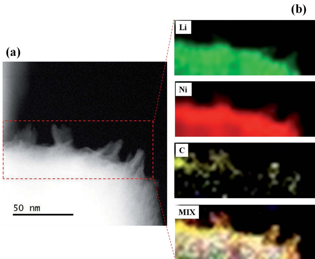
Fig. 9 (a) Typical TEM image of \text{Li}_2\text{CO}_3 (CO 2 bubbling for 7 days)-coated NCA (E-4) and (b) STEM-EELS mapping of Li, Ni and C elements and their mixed mapping.
