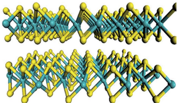
Fig. 1 The structure of MoS 2 .
