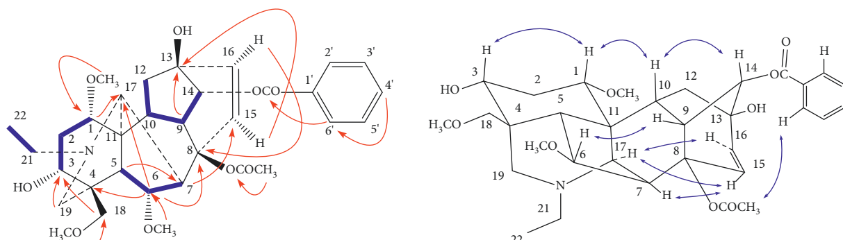
FIGURE 2: Key ^1H - ^1H COSY (—), HMBC (H→C), and NOESY (H↔H) correlations of compound 1.
