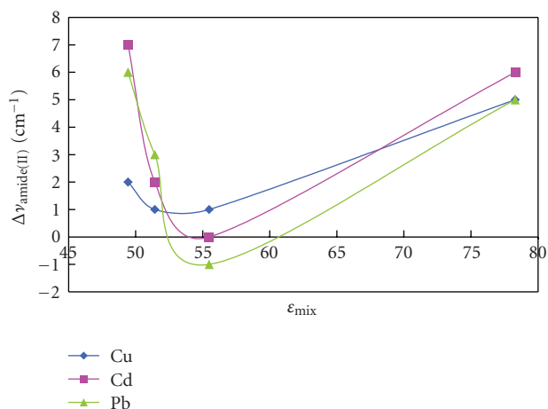
FIGURE 5: Change in amide(II) bands with \epsilon_{\text{mix}} .
