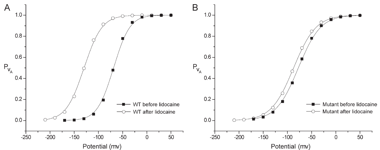
Figure 6. Simulations of fluorescence activation curves of WT and a mutant before and after the addition of lidocaine. The equations describing the probability of activation of the voltage sensor were fitted to the WT data (A) and A1145W (B) to generate the activation curves shown above (refer to Materials and methods). Symbols represent the simulated data points, and the trend lines are fits of the simulated data with a single Boltzmann function.
