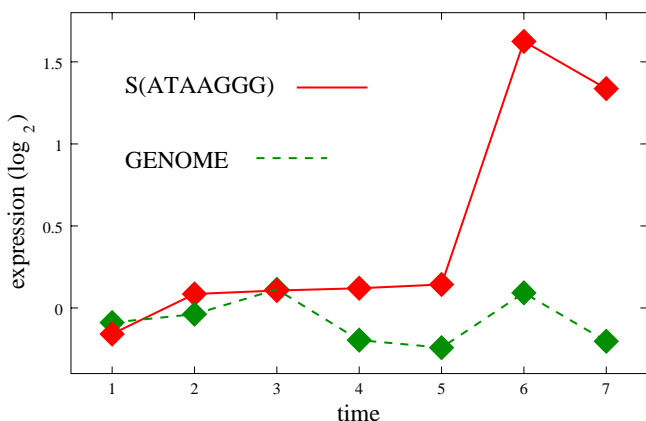
Figure 3 expression of the genes in the set S(ATAAGGG) Same as Fig. 1 for the genes in the set S(ATAAGGG), our new candidate regulatory motif.
