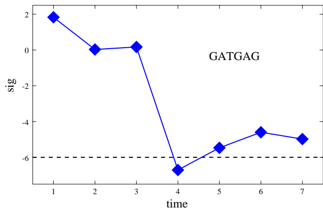
Figure 2 statistical significance of the set S(GATGAG) The statistical significance sig( i , w ) as defined in Eq. (10) for the word w = GATGAG and timepoints i = 1,..., 7 in the diauxic shift experiment. The dashed line is the significance threshold |sig| = 6.
