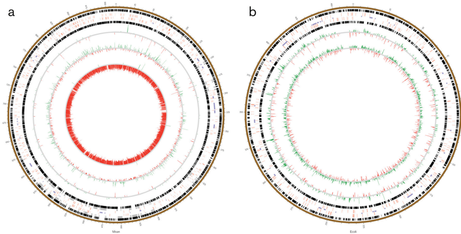
Fig. 3. Circos diagrams of the M. xanthus (a) and E. coli (b) genomes. Numbers around the diagrams each designate 10 000 bp. Black boxes represent genes encoded on the two DNA strands, red boxes designate genes encoding signalling and/or DNA-binding proteins, purple boxes are genomic islands, and grey boxes denote genes of secondary metabolite biosynthesis clusters. Nested rings represent genes differentially expressed (up-regulated in green and down-regulated in red) when comparing transcriptome datasets. The three comparisons in (a) are LIVE versus Predator Starvation (outermost), DEAD versus Predator Starvation , and Predator Nutrition versus Predator Starvation (innermost). The two comparisons in (b) are LIVE versus Prey Starvation and Prey Nutrition versus Prey Starvation .
