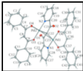
Fig. 1. The molecular structure of [\text{Pd}_2(\text{C}_{15}\text{H}_{11}\text{O}_2)_2(\text{C}_{13}\text{H}_8\text{N}_2\text{O}_2)] . Displacement ellipsoids are drawn at the 50% probability level.
