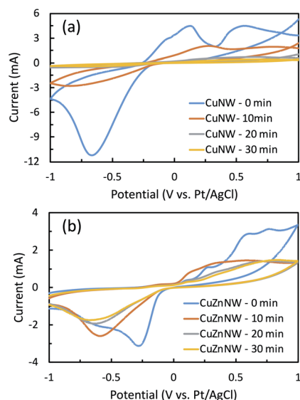
Fig. 2 Cyclic voltammograms of (a) CuNW and (b) CuZnNW. The reference electrode Ag–AgCl/saturated KCl was calibrated as 0.197 V.
