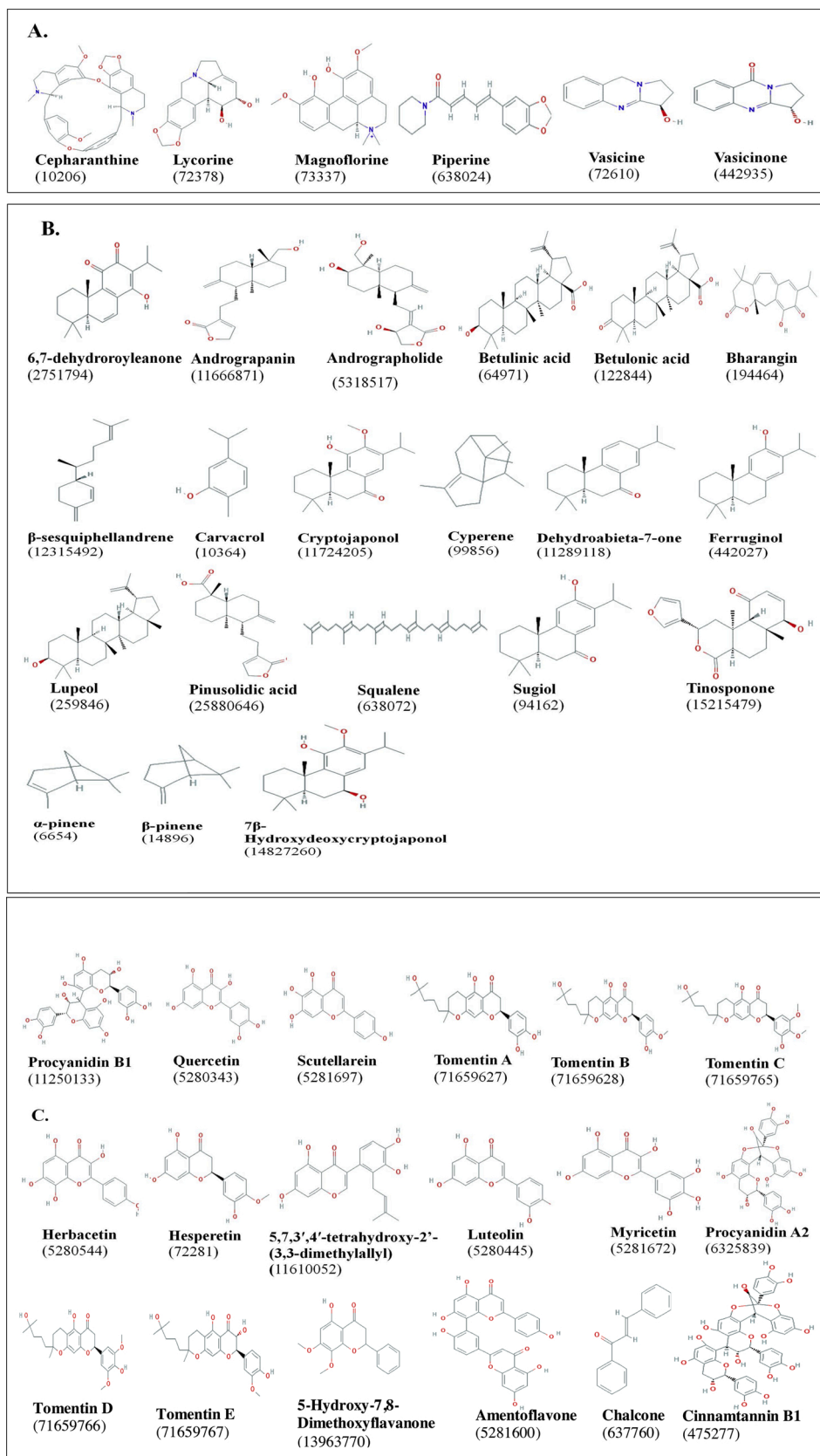
Fig. 6. Structure of various classes of phytochemicals with anti-viral potential against coronaviruses studied by in vitro , in vivo , and in silico approaches. The PubChem CID of each compound is indicated in parenthesis. A: Alkaloids; B: Terpenoids; C: Flavonoids; D: Phenolics; E: phytosterols; F: Glucosinates; G: Organosulfur compounds; H: Saponins (Source: Table 1). Structures were obtained from pubchem.ncbi.nlm.nih.gov.
