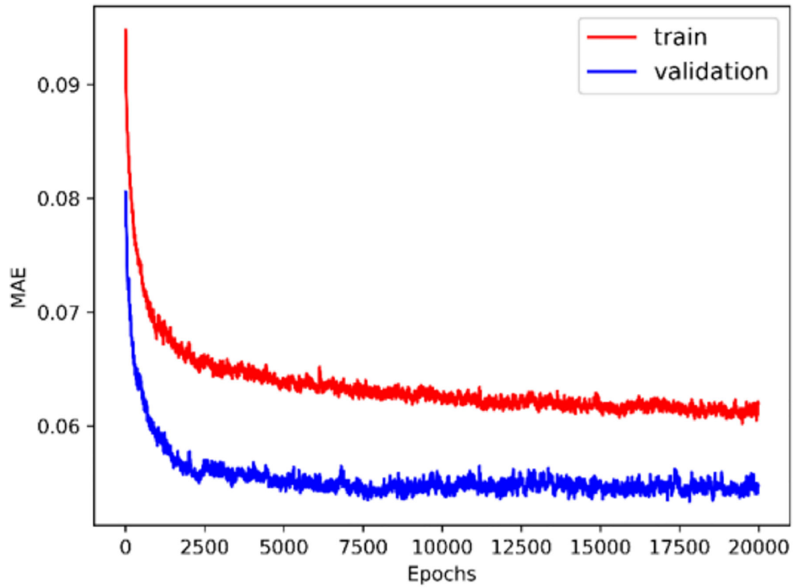
Figure 15. Five-fold cross validation results (FSI shape).
