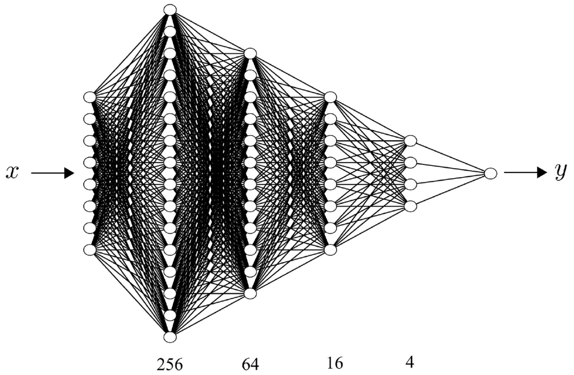
Figure 6. Architecture of the deep neural network (DNN).
