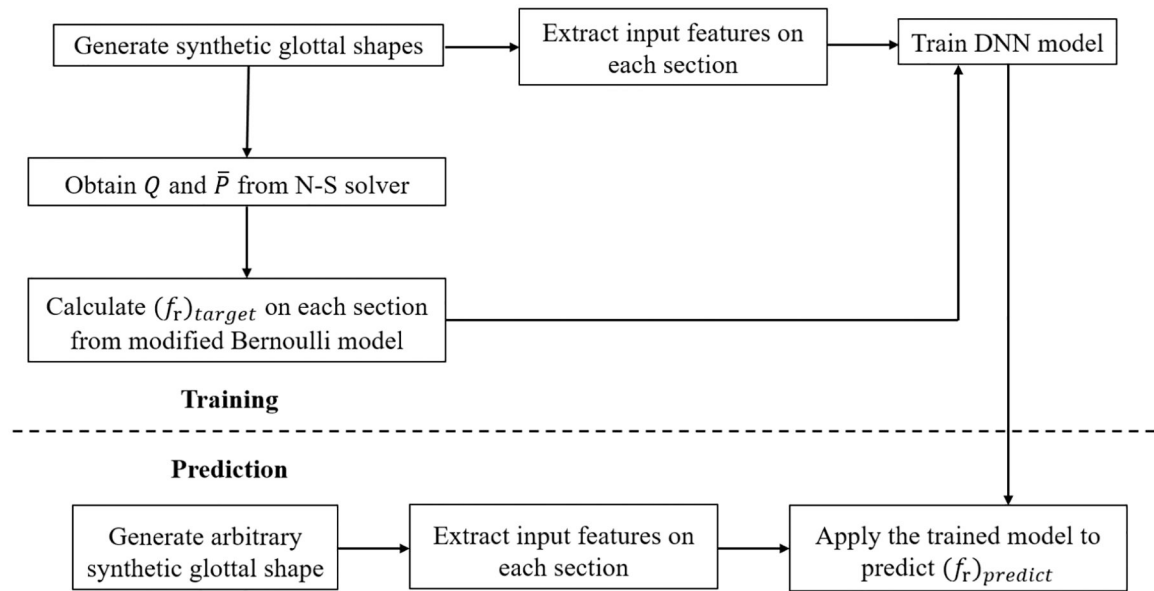
Figure 2. Workflow of training and prediction.
