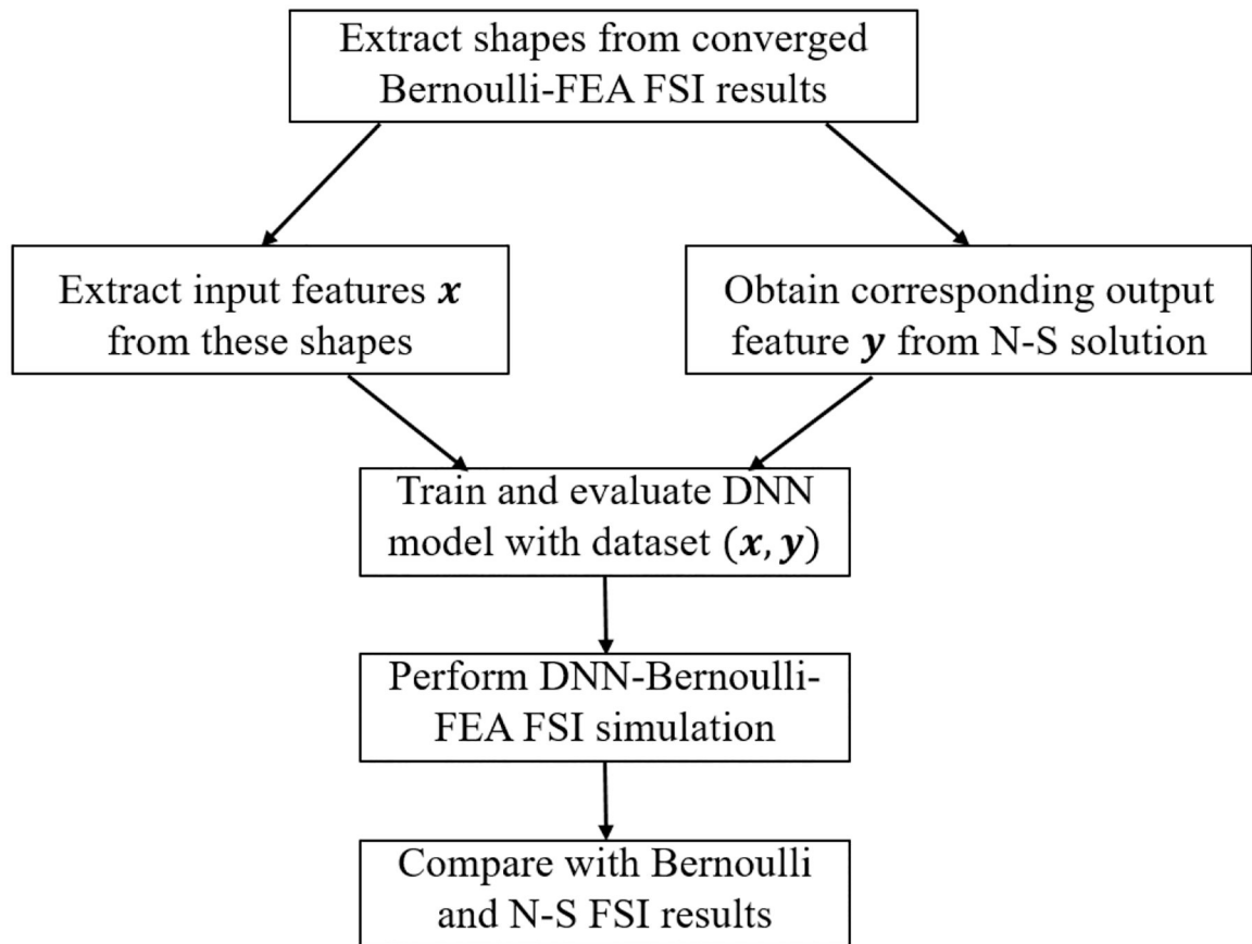
Figure 7. Workflow of the DNN-Bernoulli model for fluid structure interaction (FSI) simulation.
