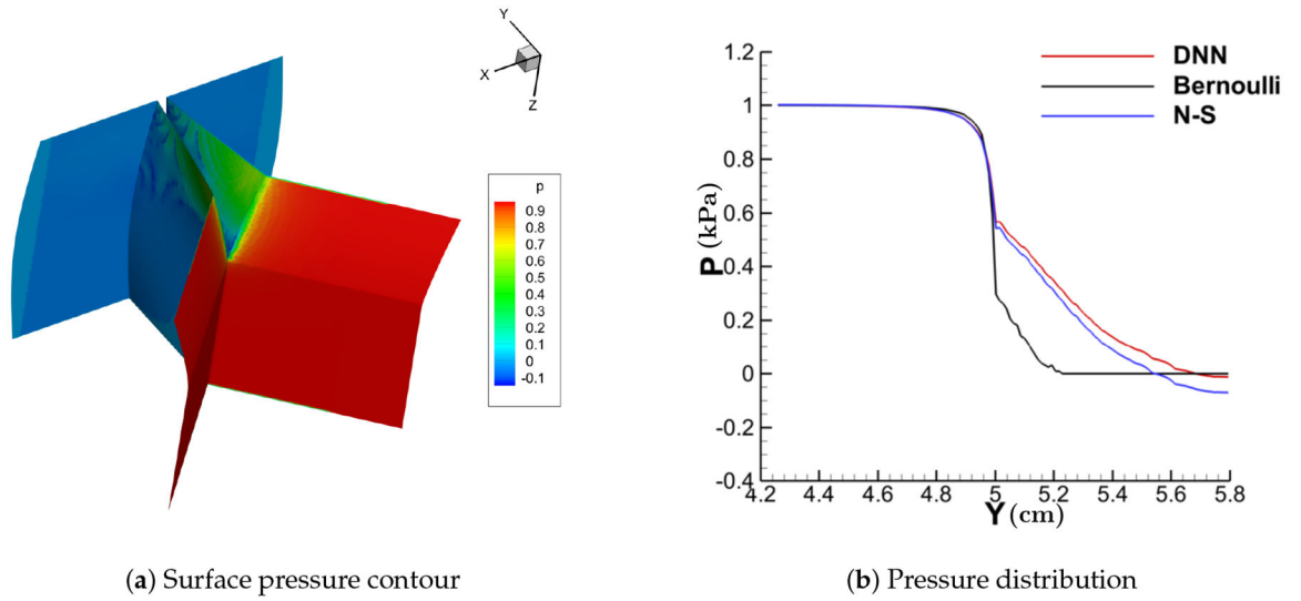
Figure 13. Surface pressure contour and distribution (convergent-divergent).
