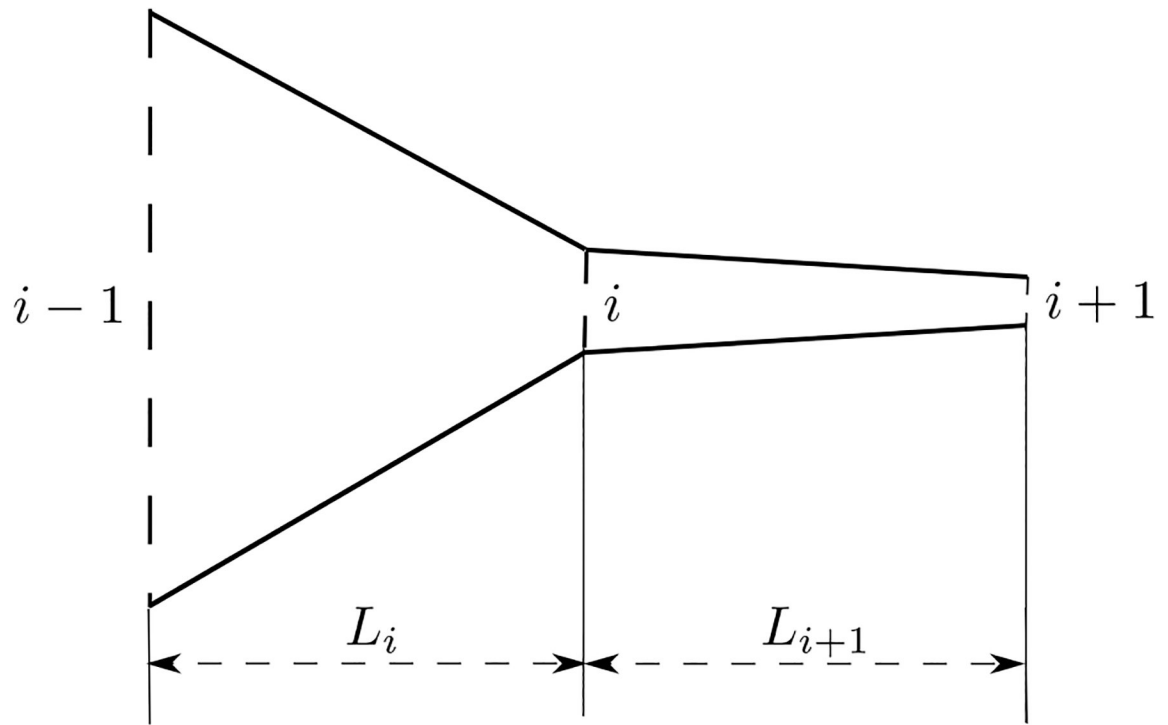
Figure 5. Schematic of discretized cross sections.
