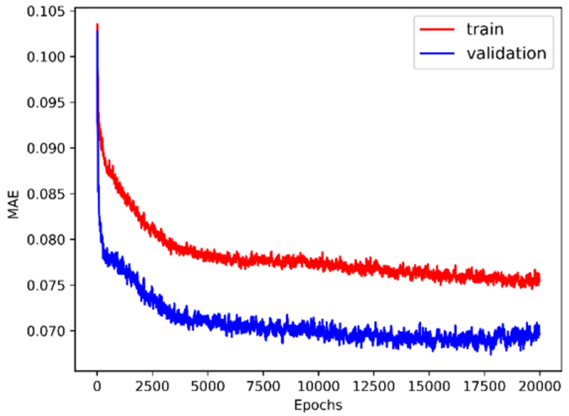
Figure 9. Five-fold cross validation results (synthetic shape).
