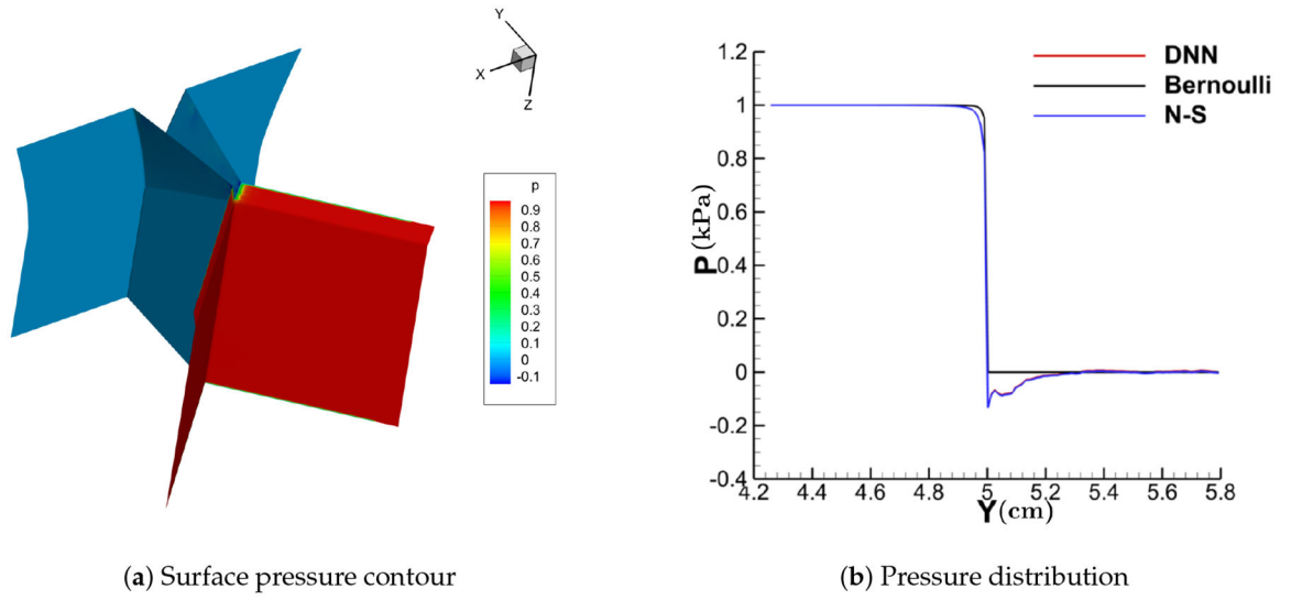
Figure 12. Surface pressure contour and distribution (divergent).
