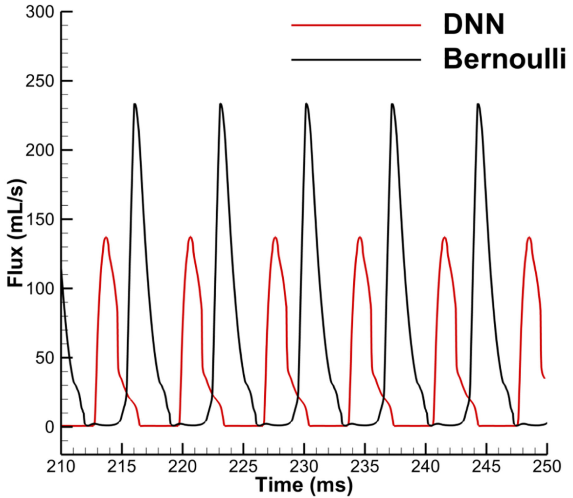
Figure 17. Comparison of the flow rate obtained by the DNN-Bernoulli and Bernoulli model.
