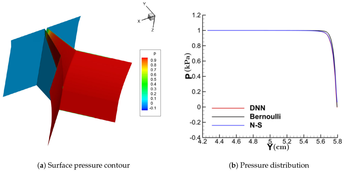
Figure 11. Surface pressure contour and distribution (convergent).
