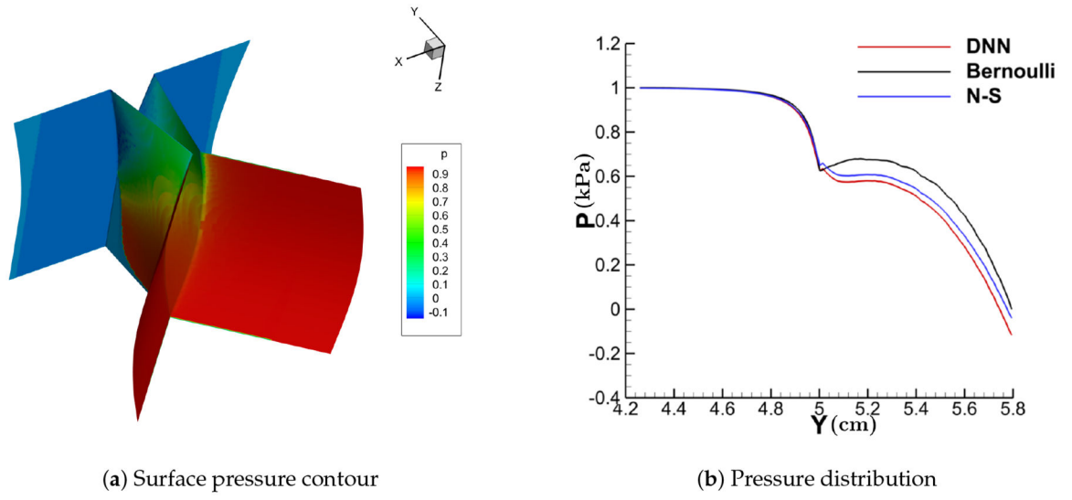
Figure 14. Surface pressure contour and distribution (divergent-convergent).
