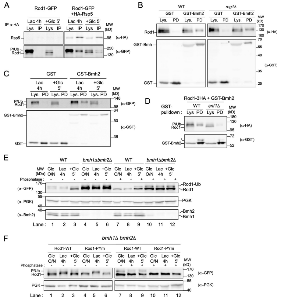
Figure 4. Rod1 ubiquitylation is regulated by a phospho-dependent binding to 14-3-3 proteins.
