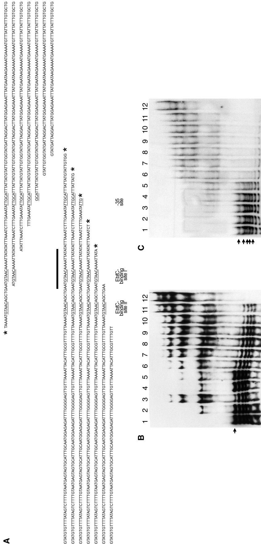
Figure 5. Identification of the high-affinity BpaB-binding site in erp Operator 2, by use of simultaneous titration of multiple probes with increasing concentrations of BpaB321. In this method, several DNAs that overlap in sequence were simultaneously incubated with protein, then subjected to EMSA. These DNAs which contain the high-affinity protein binding site were preferentially bound by lower concentrations of protein, and signals corresponding with those free DNA disappeared soonest. (A) Sequences of labeled DNA probes used in simultaneous EMSAs. Asterisks indicate DNAs preferentially bound by BpaB. The -35 sequence of the erpAB promoter and the two consensus EbflC-binding sites are indicated by underlining. The upper seven nested DNAs were anchored 51 bases downstream of the erpAB transcription start site, and EMSA data are illustrated in (B). The lower seven nested DNAs were anchored at bp -174 relative to the start of erpAB transcription, and EMSA data are illustrated in (C). Lane 1 contains only the DNAs that preferentially bound BpaB but absent from lower-affinity DNAs is indicated by a thick horizontal bar. (B) Simultaneous EMSA of recombinant BpaB321 with the upper seven DNAs of (A). Lane 1 contains only the DNAs. Lanes 2-12 contain DNAs plus increasing concentrations of recombinant BpaB321. Quantification of signal strengths indicated that BpaB bound preferentially to the largest DNA (marked with an arrowhead); in lanes 9, 10 and 12, the proportion of free DNA for this probe was 21, 0.10 and 0% of lane 1, respectively, while that of the next largest probe was 52, 13 and 10% of lane 1, respectively. (C) Simultaneous EMSA of recombinant BpaB321 with the lower seven DNAs of (A). Lane 1 contains only the DNAs. Lanes 2-12 contain DNAs plus increasing concentrations of recombinant BpaB321. Quantification of signal strengths indicated that BpaB bound preferentially to the five largest DNAs (marked with arrowheads); in lanes 7, 8 and 9, the proportion of free DNA for the largest probe was 16, 10 and 0% of lane 1, respectively, while that of the smallest probe was 75, 55 and 43% of lane 1, respectively.
