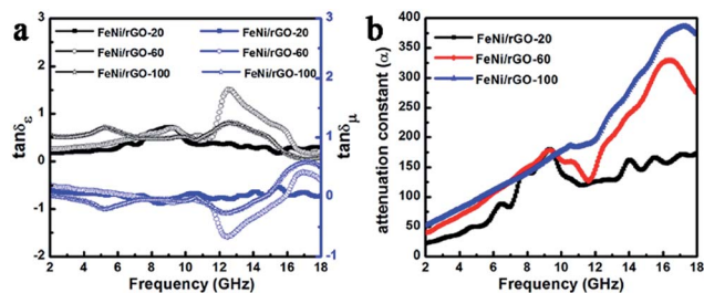
Fig. 9 Frequency dependence of \tan \delta_{\epsilon} and \tan \delta_{\mu} (a) and attenuation constant (b) of FeNi/rGO-20, FeNi/rGO-60 and FeNi/rGO-100 composites.
