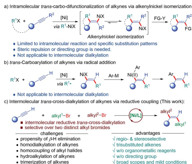
Scheme 1 Ni-catalyzed trans -selective carbo-difunctionalization of alkynes.
