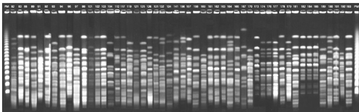
Figure 1 Pulsed-field gel electrophoresis results showing different clones of carbapenem-resistant P. aeruginosa compared with endemic clone represented by numbers 161, 162 and 163.
