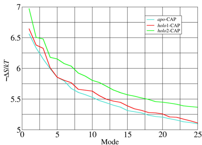
Fig. 3 Mode number for an ENM for CAP plotted against entropy ( \Delta S/kT ) for the first 25 modes. Apo-CAP ( blue ), CAP bound with one cAMP ( holo1-CAP ) ( red ), and CAP bound to two cAMP molecules ( holo2-CAP ) ( green )
