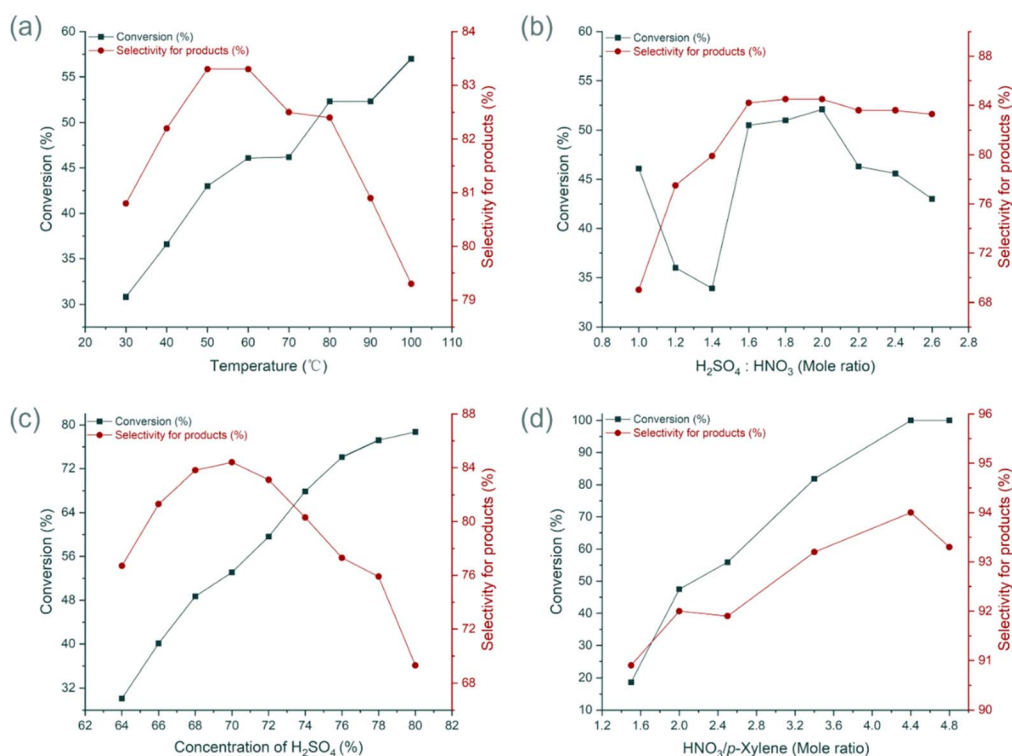
Fig. 3 Optimization of nitration in continuous-flow. (a) The influence of temperature. (b) The influence of mole ratio of H 2 SO 4 and HNO 3 . (c) The influence of H 2 SO 4 concentration. (d) The influence of mole ratio of HNO 3 and p -xylene.
