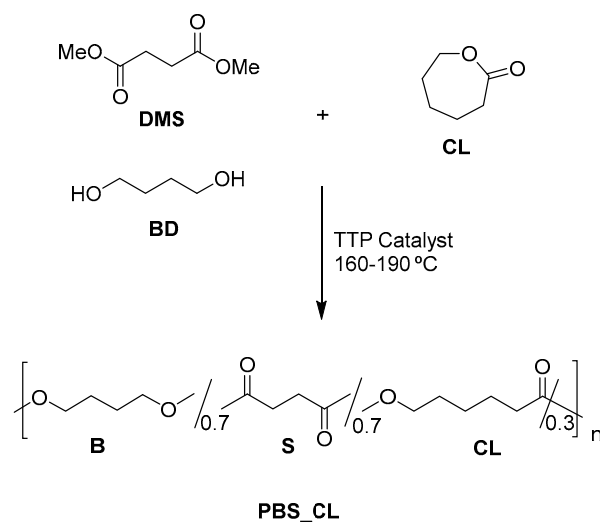
Scheme 1. Synthesis route to PBS_CL copolyester.
