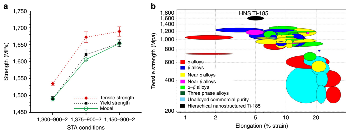
Figure 1 | Tensile strength comparison with model and other Ti alloys. (a). Ultimate tensile and yield strength of Ti185 for three STA conditions. Also shown in (a) is the prediction of empirical model in equation (2). (b) Comparison of tensile strength and strain to failure (elongation) of Ti185 alloy with other commercially available Titanium alloys. The graph in (b) is plotted using CES Selector software, Granta Design, Cambridge, UK.
