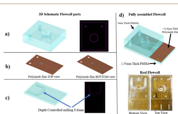
Fig. 1 Stack schematics view and real images of the flow cell. Schematic representation of (a) top PMMA element, (b) PI film including the two Ag electrodes, and (c) bottom PMMA element. (d) The schematic and real images of the fully assembled flow cell.
