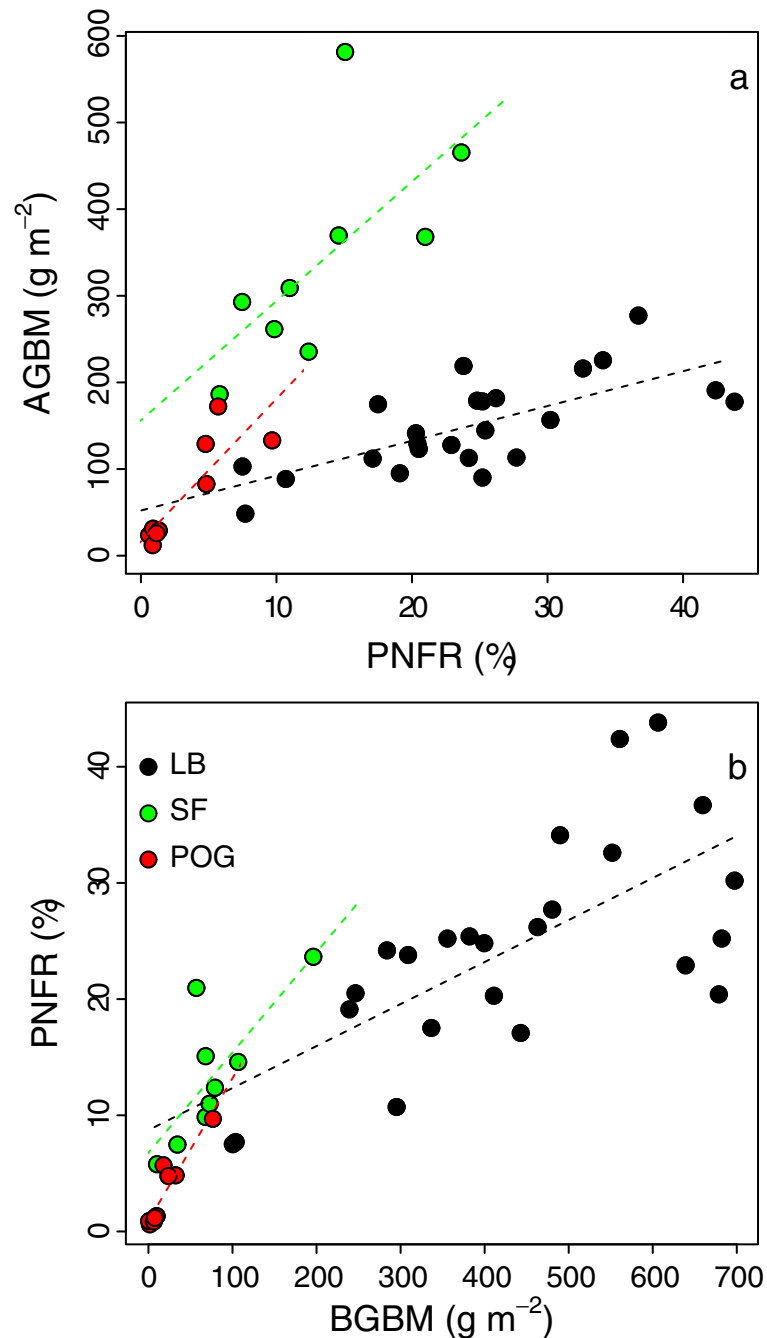
Fig 5. Relationships between the percentage of fertilizer-derived N recovered (PFNR) and aboveground biomass (AGBM; g m -2 ) and belowground biomass (BGBM; g m -2 ) in the three study plant species. (a) Relationship between PFNR and AGBM; y = 52.12 + 4.02x ( R^2 = 0.49 ; P < 0.001 ) for LB; y = 156.2 + 13.77x ( R^2 = 0.44 ; P = 0.05 ) for SF; y = 16.38 + 16.46x ( R^2 = 0.74 ; P = 0.005 ) for POG. (b) Relationship between BGBM and PFNR; y = 8.72 + 0.036x ( R^2 = 0.47 ; P < 0.001 ) for LB; y = 6.77 + 0.086x ( R^2 = 0.58 ; P < 0.05 ) for SF; y = 0.91 + 0.123x ( R^2 = 0.87 ; P < 0.001 ) for POG. LB, SF and POG stand for lowbush blueberry, sweet fern and poverty oat grass, respectively.
