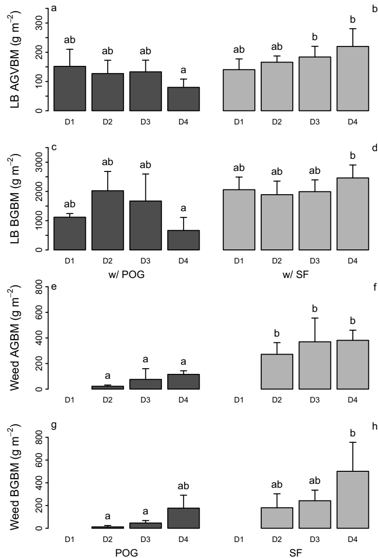
Fig 1. Aboveground vegetative biomass (AGVBM) production and belowground biomass (BGBM) ( \text{g m}^{-2} ) in the three study plant species. (a–d) AGVBM and BGBM in lowbush blueberry (LB) in mixtures with poverty oat grass (POG; dark grey bars) or sweet fern (SF; light grey bars). (e–h) AGVBM and BGBM in POG (dark grey bars) or SF (light grey bars) in mixtures with LB. Values are mean \pm SD ( n = 3 ) and are shown for the four levels of weed density (D1–D4). Values not sharing the same letters are significantly different at P < 0.05 .
