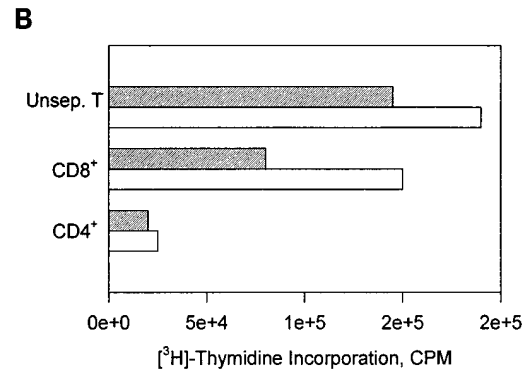
Figure 3. (A) Anti-4-1BB mAbs differentially costimulate in vitro proliferation of CD4 + and CD8 + T cell subsets. Purified resting CD4 + or CD8 + BALB/c splenic T cells were cultured for 72 h in 96-well microtiter plates at 1 \times 10^5 /well with 0.5% APC \pm anti-4-1BB mAb at 10 \mu g/ml and the indicated concentration of anti-CD3 mAb. Cells were pulsed with 0.5 \mu Ci/well [ 3 H]thymidine for the final 12 h of culture, harvested, and counted by liquid scintillation spectroscopy. (B) 4-1BB-Ig fusion protein inhibits anti-CD3-induced T cell proliferation. CD4 + and CD8 + T cells with APC were stimulated with anti-CD3 mAb at 300
