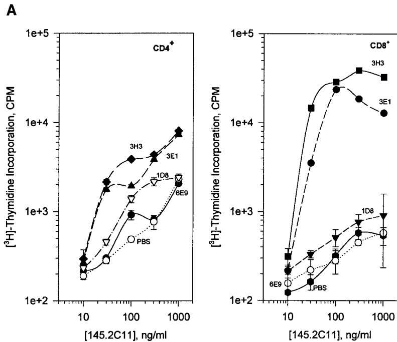
ng/ml in the absence or presence of soluble 4-1BB-Ig fusion protein. Cells were pulsed during the final 12 h of culture with [ 3 H]thymidine, harvested, and counted by liquid scintillation spectroscopy.
