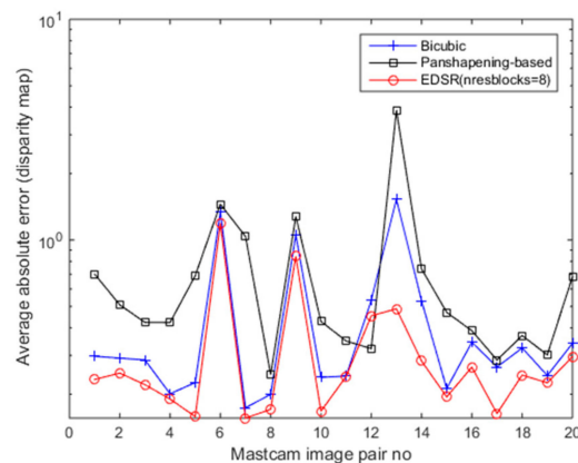
Figure 20. Average absolute errors for 20 Mastcam image pairs.
