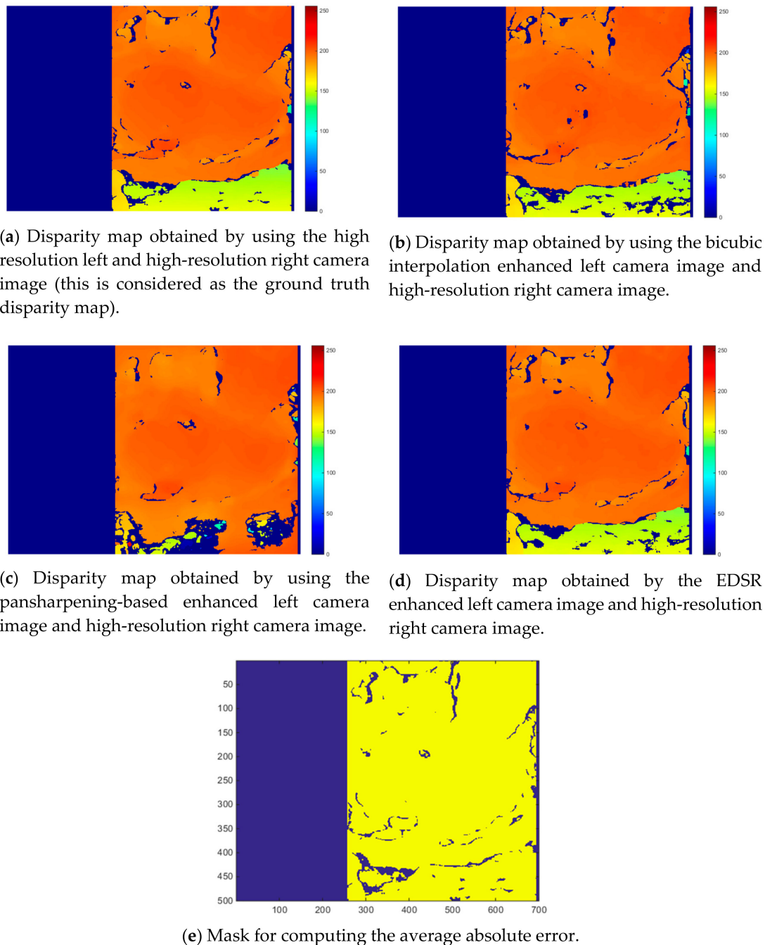
Figure 8. Disparity map estimations with the three methods and the mask for computing average absolute error.
