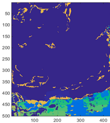
(c) Absolute disparity map difference between the ground truth disparity map and the disparity map obtained by using the pansharpening-enhanced left camera image (average absolute error = 17.5770).
