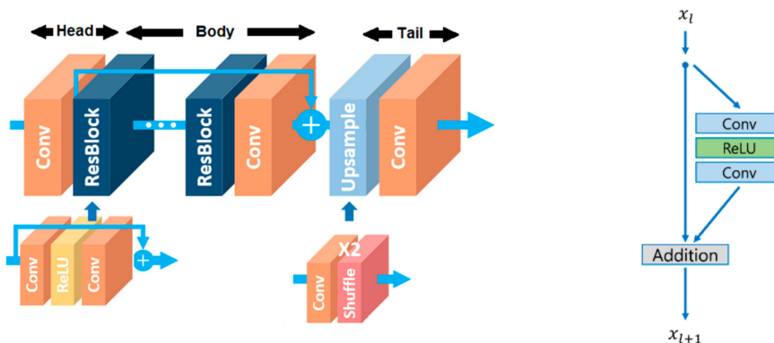
(a) Enhanced deep super resolution (EDSR) architecture (single-scale) (b) Residual block
