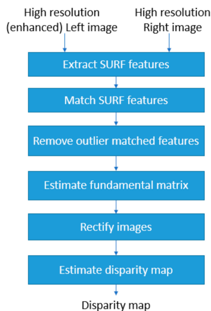
Figure 6. Processing steps of the disparity map estimation.
