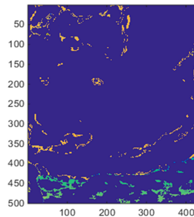
(d) Absolute disparity map difference between the ground truth disparity map and the disparity map obtained by using the EDSR-enhanced left camera image (average absolute error = 5.1492).
