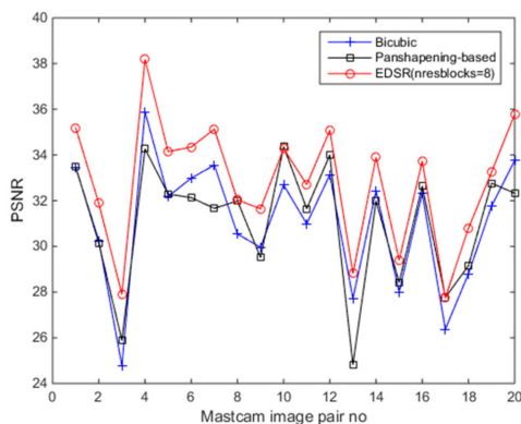
(c) PSNR (higher score is better).
