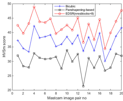
(e) HVSm (higher score is better).
