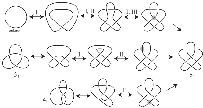
Figure 7. Three ways \overline{6_2} can be formed via a single crossing change. This shows how one crossing change on the unknot, \overline{3_1} or 4_1 can result in the knot \overline{6_2} . The double arrows indicate moves that do not change the knot type; they are the Reidemeister moves I, II and III and planar isotopies. The single arrow indicates when a crossing change is made at the highlighted crossing.
