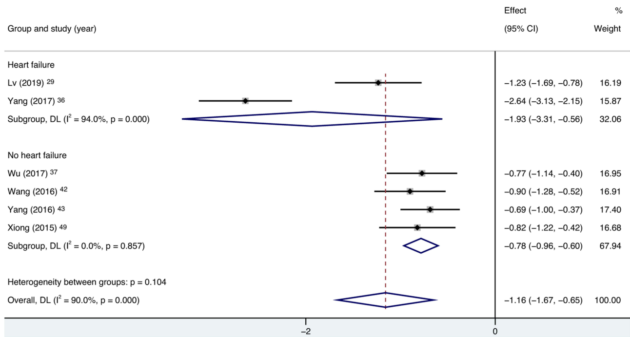
Figure 10 Forest plot of IL-6, subgroup analysis was performed according to variable of heart failure and no heart failure.
