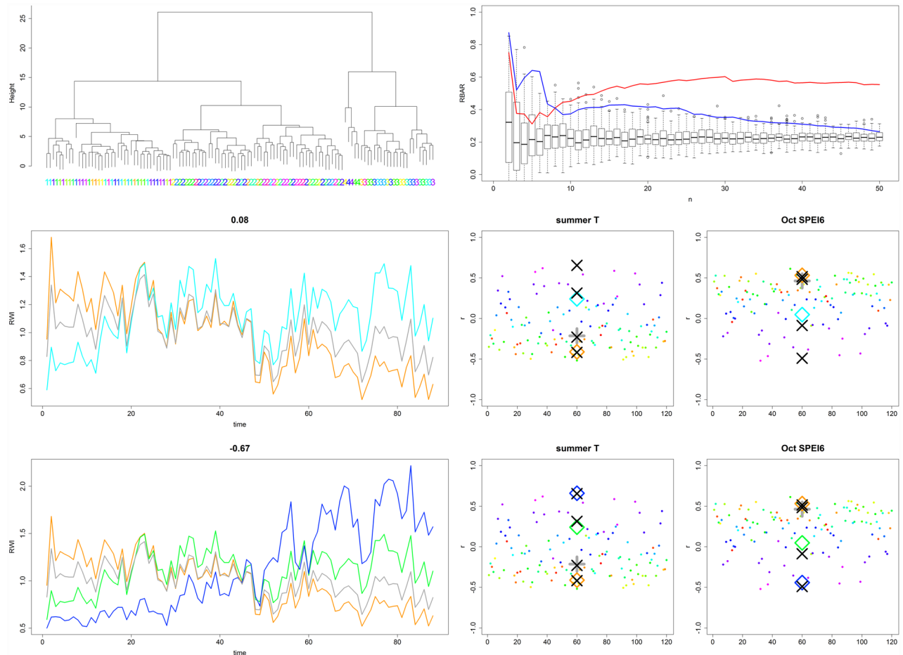
Fig 8. Evaluations plots for BR:FO. Upper left: HCA dendrogram suggests selection of four responder chronologies. Note, that cluster four only consists of five specimens. Upper right: g\bar{r}bar_N clearly indicates signal strength enhancement at the margins of the population. Mid left: PCGA extreme responder chronologies show weak correlations with each other. Mid right: PCGA and HCA responder chronology signal correlations are comparably strong: see also Table 2. Lower left: Same as mid-left but here for the analyses where the minimum sample size was adjusted to match HCA minimum sample size. Lower right: Same as mid right but here for the analyses where the minimum sample size was adjusted to match HCA minimum sample size.
