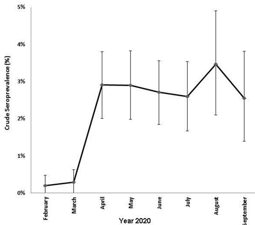
Fig. 2. SARS-CoV-2 antibody detection in donations received between February 2020 and September 2020. Error bars represent 95% confidence intervals.
