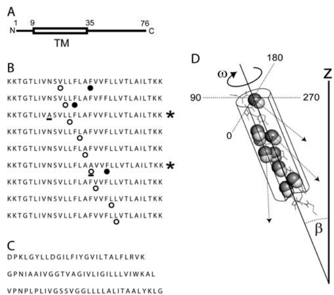
FIGURE 1 (A) Position of the putative TMH domain (TM, see box) in the complete sequence of SARS-CoV E. The residue numbers and N- and C-termini are indicated. (B) Peptides synthesized corresponding to ETM, labeled at various positions with ^{13}\text{C}=\text{O} (○) and cyano-phenylalanine (●); two mutated sequences are indicated with a star (right), and the mutated residues are underlined. (C) Synthetic peptides used as a control, corresponding to the TMH domain of CD3- \zeta (top), integrin \beta 2 (middle), and integrin \alpha M (bottom). (D) Schematic representation of an \alpha -helix with parameters \omega (range 0\text{--}359^\circ ) and \beta (range 0\text{--}90^\circ ). The peptidic C=O bonds isotopically labeled are shown as spheres (C, solid; O, open). The arrows indicate the direction of the C=O bond relative to the z axis. This direction is obtained from the helix and label dichroic ratios (see Experimental Procedures) and is used to determine \omega .
