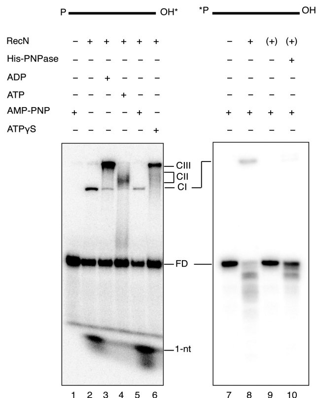
Figure 1. 3'-to-5' ssDNA exonuclease activity in the RecN sample. Linear ssDNA 60 (1 nM), labelled (*) at the 3'-end (lanes 1–6) or the 5'-end (lanes 7–10) was incubated with RecN (10 nM) purified from wt cells or from the \Delta pnpA strain [denoted as (+)] in buffer B for 10 min at 37^{\circ}\text{C} . Where indicated, ADP, ATP, AMP-PNP or ATP \gamma S (1 mM) was added and incubation continued for 30 min at 37^{\circ}\text{C} . For the reaction shown in lane 10, His-PNPase (0.1 nM) was added after 10 min to the pre-formed RecN-ssDNA 60 complex. Incubation products were separated in 10% nPAGE and visualized by autoradiography. RecN-ssDNA complexes are labelled CI, complex I; CII, complex II; CIII, complex III (14,15); FD, free DNA. Migration of [ 32 P]-labelled mononucleotide released by incubation with RecN is indicated (1 nt).
