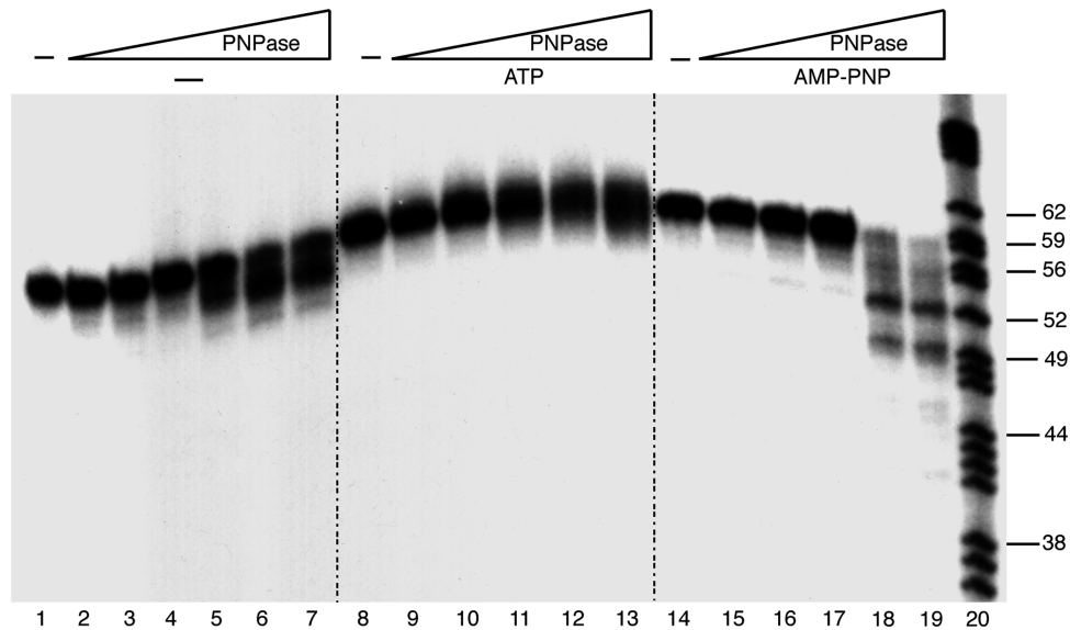
Figure 4. PNPase promotes limited degradation of ssDNA. [ ^{32} P]-ssDNA 60 (1 nM) was incubated with increasing concentrations of PNPase (0.02, 0.04, 0.08, 0.16, 0.33 and 0.66 nM) for 30 min in buffer B containing 1 mM ATP, AMP-PNP or lacking a nucleotide cofactor, and the samples were separated in 15% dPAGE. Sizes of molecular markers (in nt) are indicated (lane 20).
