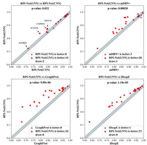
Fig. 3. Comparison of RPI-Net(GNN) ROC AUC values to previous models and RPI-Net(CNN). The dotted lines correspond to a 1% difference. The P -value is calculated for the Wilcoxon signed-rank test with the alternative hypothesis that AUC scores of RPI-Net(GNN) are greater
