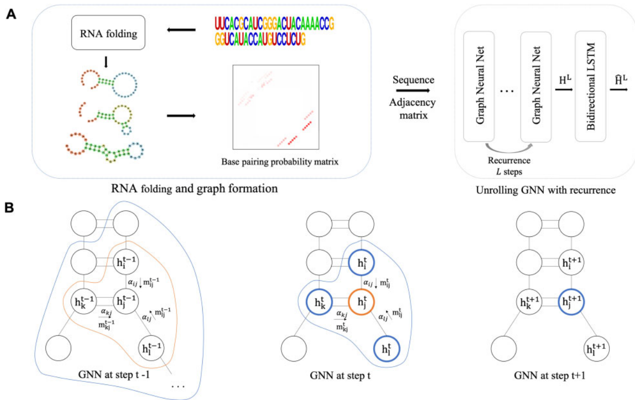
Fig. 1. (A) Our GNN model takes in as input an adjacency matrix that specifies the base-pairing probabilities, as well as the one-hot encoded nucleotide sequence. The message passing layers are unrolled L steps using a LSTM model (Hochreiter and Schmidhuber, 1997), whose output is then fed to a bidirectional LSTM module to learn a more global nucleotide embedding. (B) Here, we show an example of message passing to node j from its 2-hops neighborhood. m_{ij} denotes the messages passed from node i to j , and to keep the notation uncluttered we have omitted its type and direction. \alpha_{ij} is a scalar used for the base-pairing probability when m_{ij} is passed along a hydrogen bond, otherwise it is set to one. The node features associated to j at time step t is denoted as h_j^t , and it is updated with the information from its adjacent nodes according to Equations (2)–(4)
