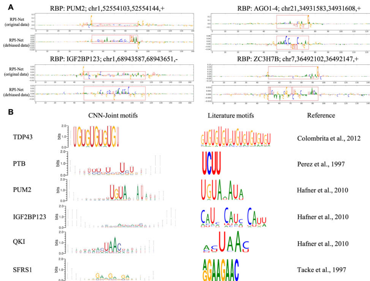
Fig. 4. Integrated gradient maps and sequence motifs obtained using RPI-Net(CNN). (A) Integrated gradient values for four positive examples, revealing that debiasing the CLIP-Seq data is crucial for RPI-Net(CNN) to learn meaningful protein binding hypothesis. When RPI-Net is trained on the original (biased) datasets, the border artefacts will receive the highest attribution of the model's prediction. Trained on debiased datasets, the border artefacts are eliminated and meaningful protein binding pattern are revealed inside the viewpoint region (enclosed red rectangles). (B) Shows six sequence logos extracted from RPI-Net(CNN) models, compared to the known motifs for those RBPs. The widths of characters become smaller as more gaps are inserted to that position. Our sequence motifs have shown a strong agreement to the literature motifs that are experimentally verified. Image credits: The literature motif images are taken from Maticzka et al. (2014) , Figure 5
