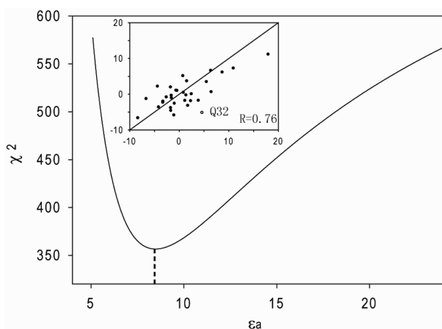
Figure 3. \chi^2 fitting error of CSPs as a function of \epsilon_a , with \chi^2 = \sum(\Delta\delta_{\text{pred}} - \Delta\delta_{\text{exp}})^2 , excluding the outlier Q32, at 298 K. The minimum \chi^2 is obtained for \epsilon_a = 8.6 .
