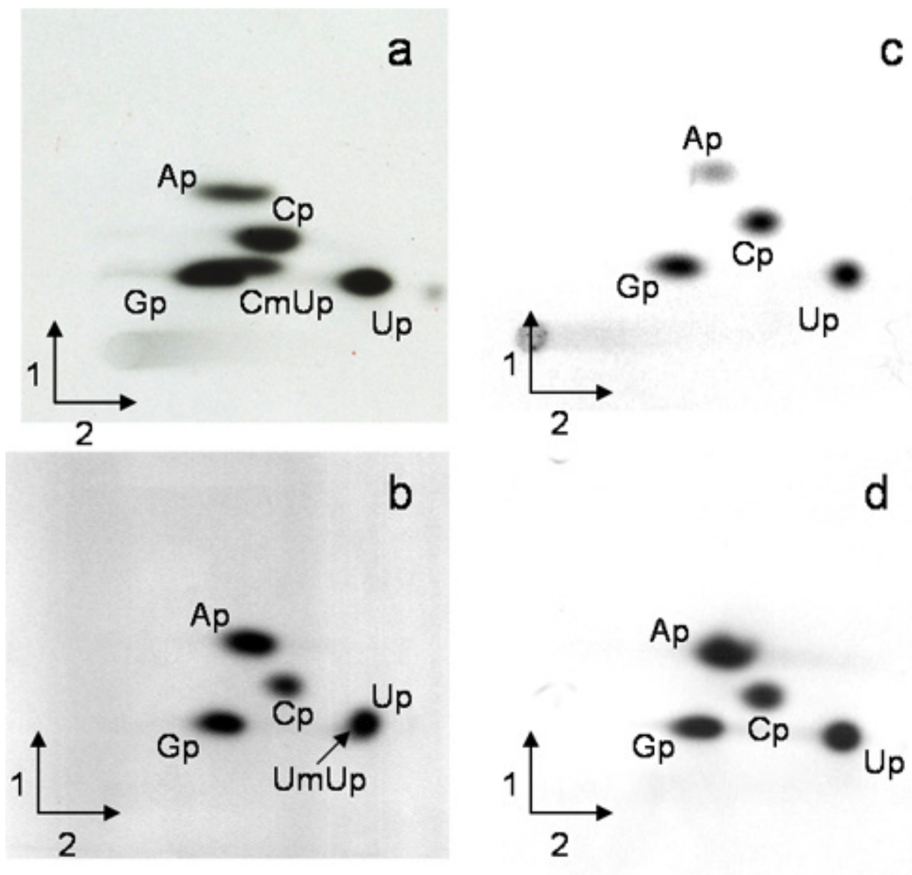
Figure 5 RNase T2 cleavage of in vitro transcribed E. coli tRNA SerI and tRNA Gln2 incubated with YfhQ and AdoMet. Autoradiography of two-dimensional chromatograms of 5'-phosphate and 3'-phosphate nucleosides on thin layer cellulose plates. [ \alpha - 32 P]UTP-labelled in vitro transcribed tRNA SerI ( 2.5 \times 10^5 cpm) (a and c) and [ \alpha - 32 P]UTP-labelled in vitro transcribed tRNA Gln2 ( 2.5 \times 10^5 cpm) (b and d) was incubated in the presence (a and b) or absence (c and d) of the YfhQ protein. The reaction mixture contained 50 mM PIPES-Na, pH 7.0, 4 mM MgCl 2 , 50 \mu M AdoMet and 5 \mu g of the purified YfhQ protein. After 90 min incubation at 37°C, the tRNA was recovered, cleaved by RNase T2, the resulting nucleotides were analyzed as described [38].
