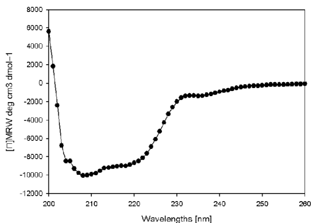
Figure 12 Far UV CD spectrum of YfhQ protein. Spectra were measured in 0.15 M Tris-HCl pH7.5 buffer and corrected by subtraction of a buffer spectrum. The concentration of YfhQ protein was 6.6 μM. Three accumulations were measured, which were recorded in millidegrees every 1 nm. The mean residue ellipticities for the spectra were calculated to aid in secondary structure determination by comparison with standard spectra for secondary structure elements.
