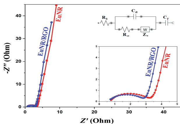
Fig. 9 Impedance spectra of EuNR and EuNR-RGO. The frequency range is 0.1-10^5 Hz.
