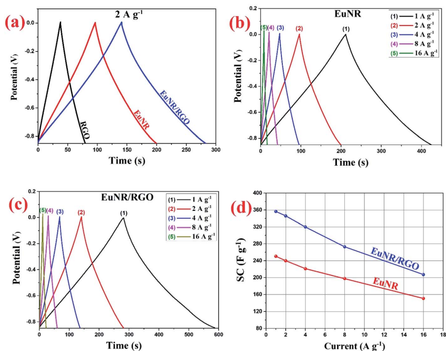
Fig. 7 (a) RGO, EuNR and EuNR-RGO charge/discharge curves at 2.0 \text{ A g}^{-1} current density; (b) EuNR charge/discharge curves at 1\text{--}16 \text{ A g}^{-1} current densities; (c) EuNR-RGO charge/discharge curves at 1\text{--}16 \text{ A g}^{-1} current densities and (d) EuNR and EuNR-RGO specific capacitance changes with changing current densities from 1 to 16 \text{ A g}^{-1} .
