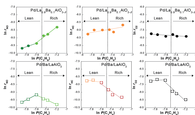
Fig. 3 Dependence of the reaction rate on the partial pressure of \text{C}_3\text{H}_6 on \text{Pd}/\text{La}_{0.9}\text{Ba}_{0.1}\text{AlO}_{3-\delta} and \text{Pd}/\text{Ba}/\text{LaAlO}_3 at 523\text{ K} during \text{NO-C}_3\text{H}_6\text{-O}_2\text{-H}_2\text{O} reaction.
